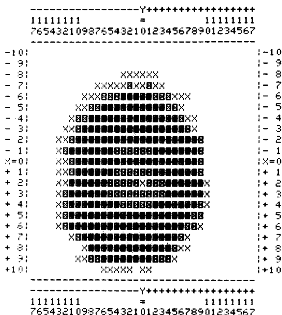
Fig.2. Optical density map of a single erythrocyte at pH 7.2 fully saturated with carbon monoxide ( [CO] 10^{-3} M). Observation wavelength \lambda = 415 nm.
