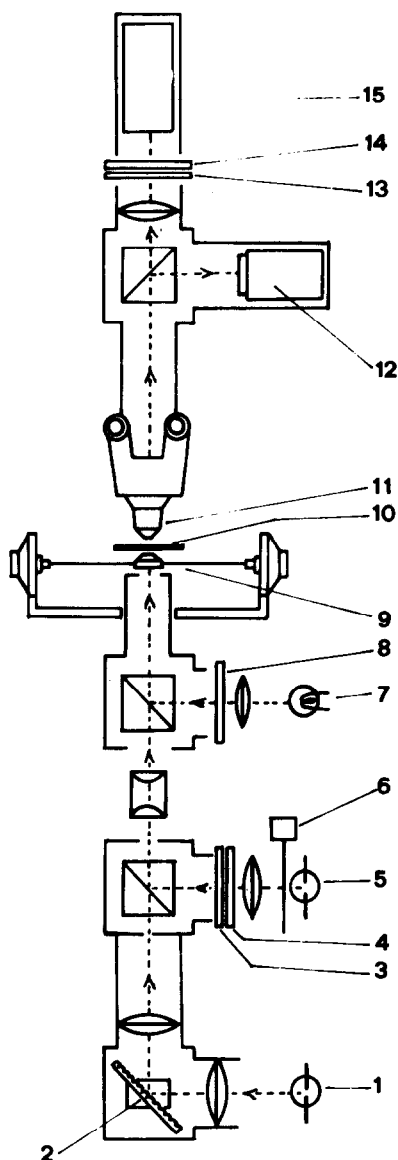
Fig.1. Configuration of the apparatus as used for the experiments described in this paper. (1) Xenon arc lamp XBO 75 W2-2) Grating monochromator. (2) Absorption filter (Schott, BG 38, 4 mm). (4) Interferential filter (Balzers, \lambda = 546 nm). (5) Mercury arc lamp, HBO 100 W2. (6) Electromechanical shutter. (7) Tungsten lamp. (8) Infrared filter. (9) Moving-condenser unit (70 \times 0.90 dry). (10) Sample carrier. (11) Collection optics. (12) Infrared video camera. (13) Filter (Schott, BG 12, 3 mm). (14) Interference filter (Balzers FITC 3). (15) Photomultiplier tube (EMI 96588).
